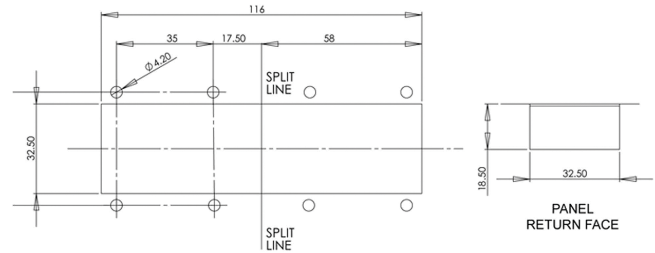
Panel cut-out
