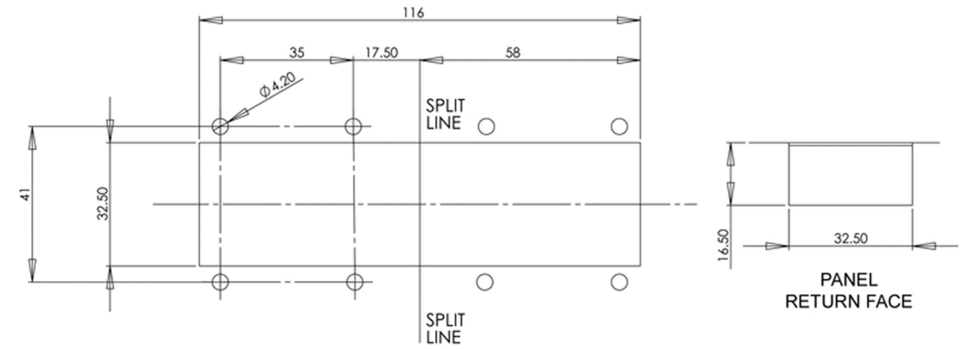
Panel cut-out
