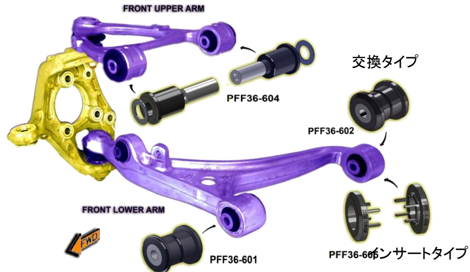
Mazda MX5 Mk 4 ND (2015 - ) FRONT SUSPENSION BUSHES
