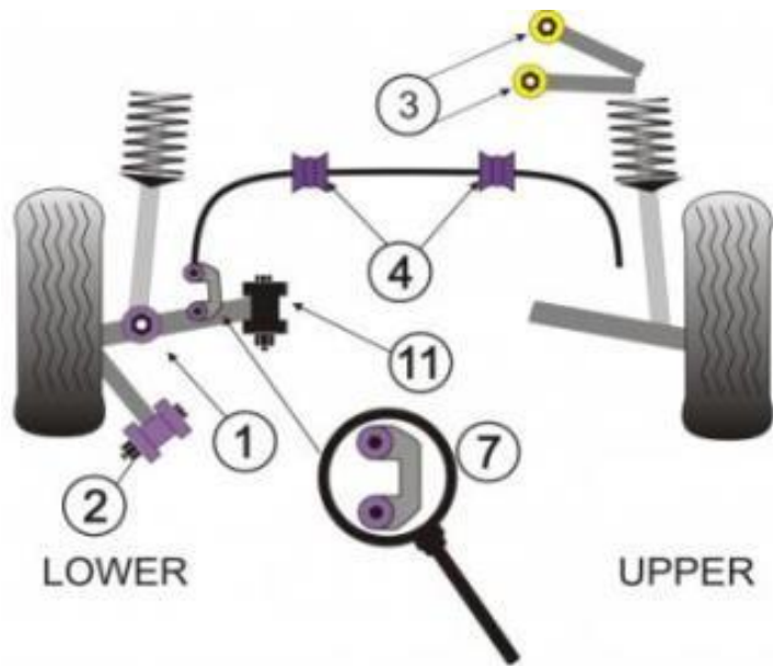
A4, S4, RS4, QUATTRO Platform B5 Type 8D
